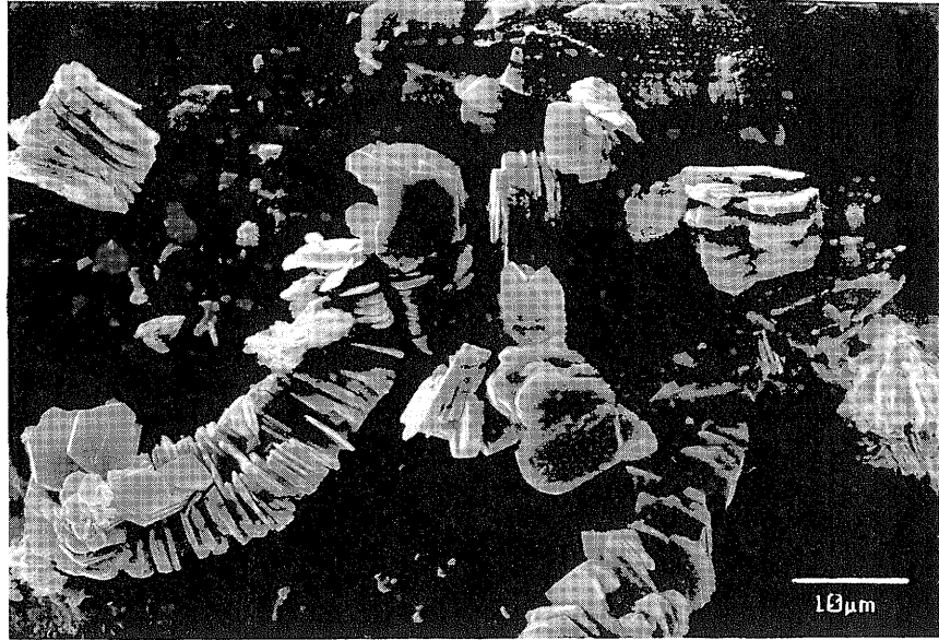
Figure 15 SEM photomicrograph shows kaolinite crystals on a quartz overgrowth substrate. The kaolinite booklets are loosely bound to the quartz grain. The sample is from the Cypress C sandstone reservoir of the Droege Unit No. 2 (1,505 feet).
