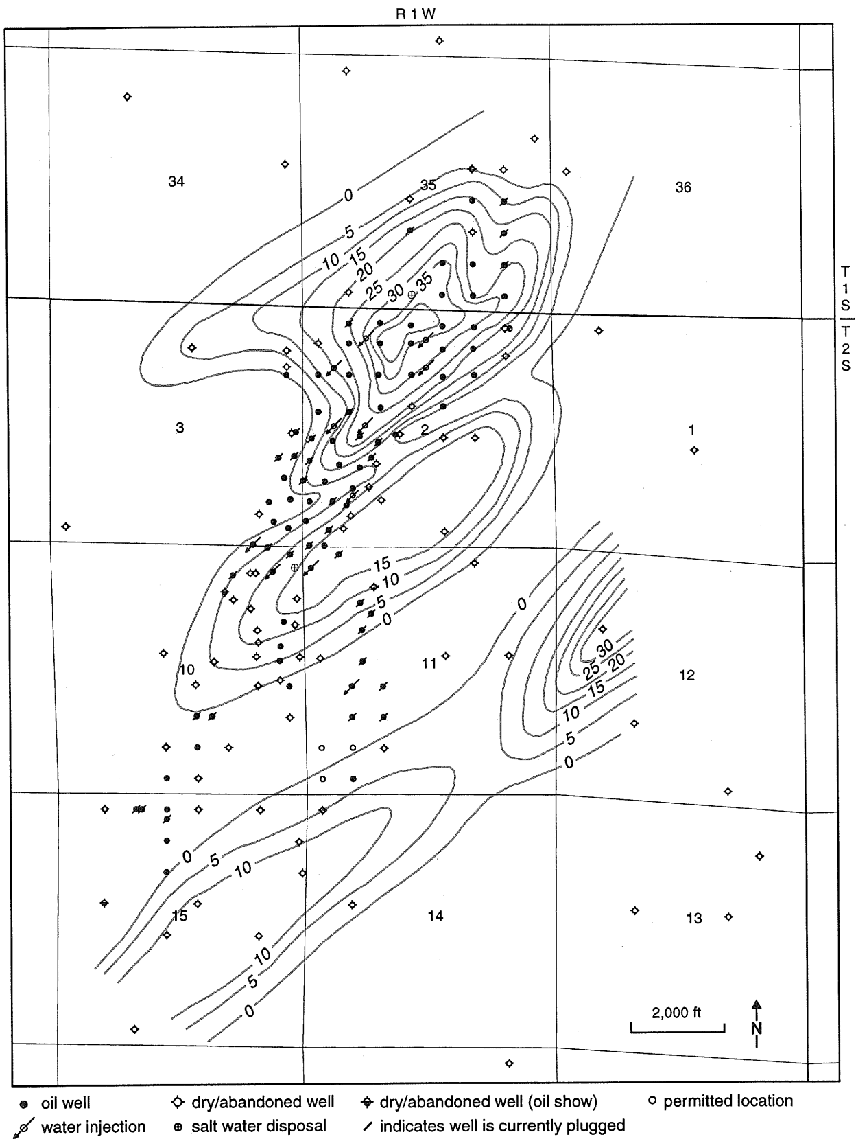
Figure 7 Net thickness map of the Cypress A sandstone that is greater than 50% clean. Contour interval is 5 feet.
