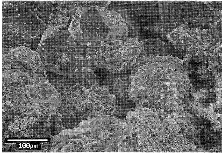
Figure 13 SEM photomicrograph shows angular sand grains resulting from quartz overgrowths. Several pore throats in the center of the photomicrograph are restricted by overgrowths. In the lower part of the image, clay minerals coat the sand grains and appear to retard quartz overgrowths. Sample is from the Cypress C sandstone reservoir of the Droege Unit No. 2 (1,505.5 feet).
