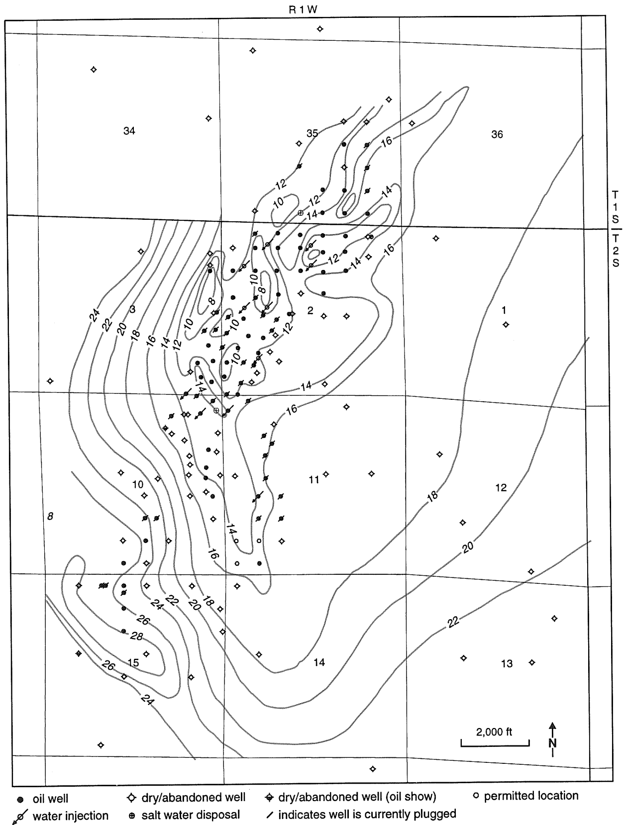
Figure 12 Thickness map of the Beech Creek (Barlow) Limestone. Contour interval is 2 feet. The Cypress consists predominantly of sandstones where the Barlow is thin.
