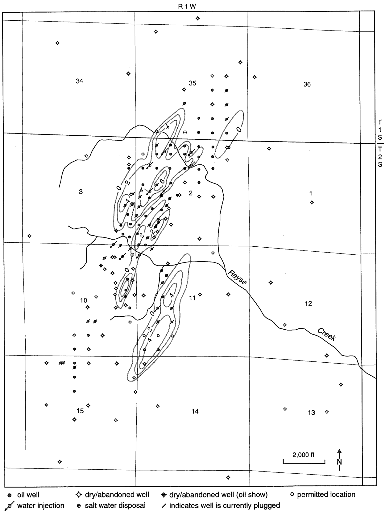
Figure 11 Net thickness map of the Cypress D sandstone showing multiple, lenticular sandstones trending northeast-southwest. Contour interval is 2 feet.
