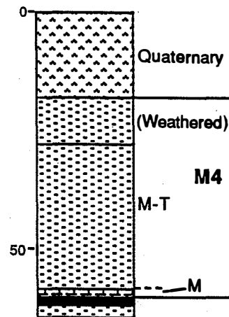
Figure 6. Graphic column of cyclothem M4 from borehole G-08.
