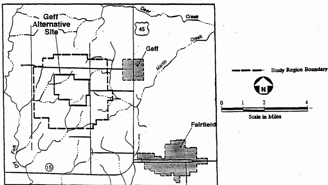
Figure 1. Upper map shows location of drill holes at the Geff Alternative Site used in this study. Lower map shows location of site in the west-central portion of Wayne County.
