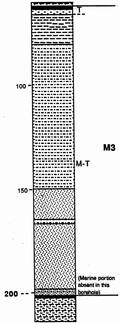
Figure 5. Graphic column of cyclothem M3 from borehole G-08.
