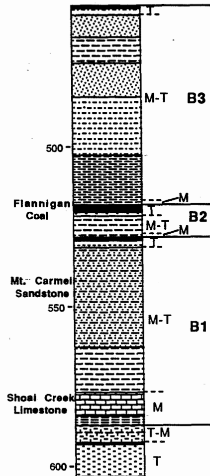
Figure 2. Graphic column of cyclothems B1, B2, and B3 from borehole G-08.
