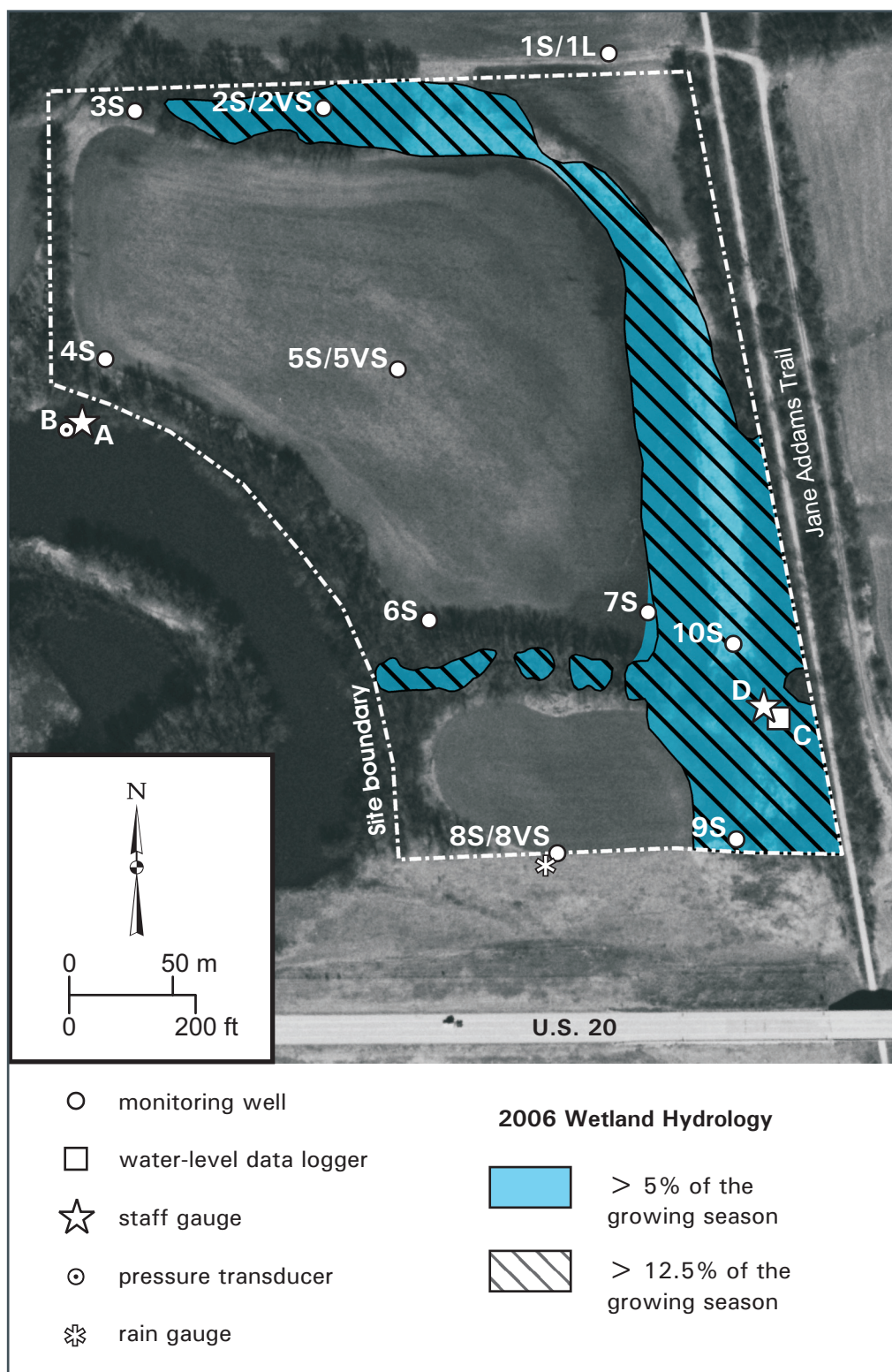
Figure F3 Areas exhibiting wetland hydrology in 2006 (map based on ISGS 2006).
