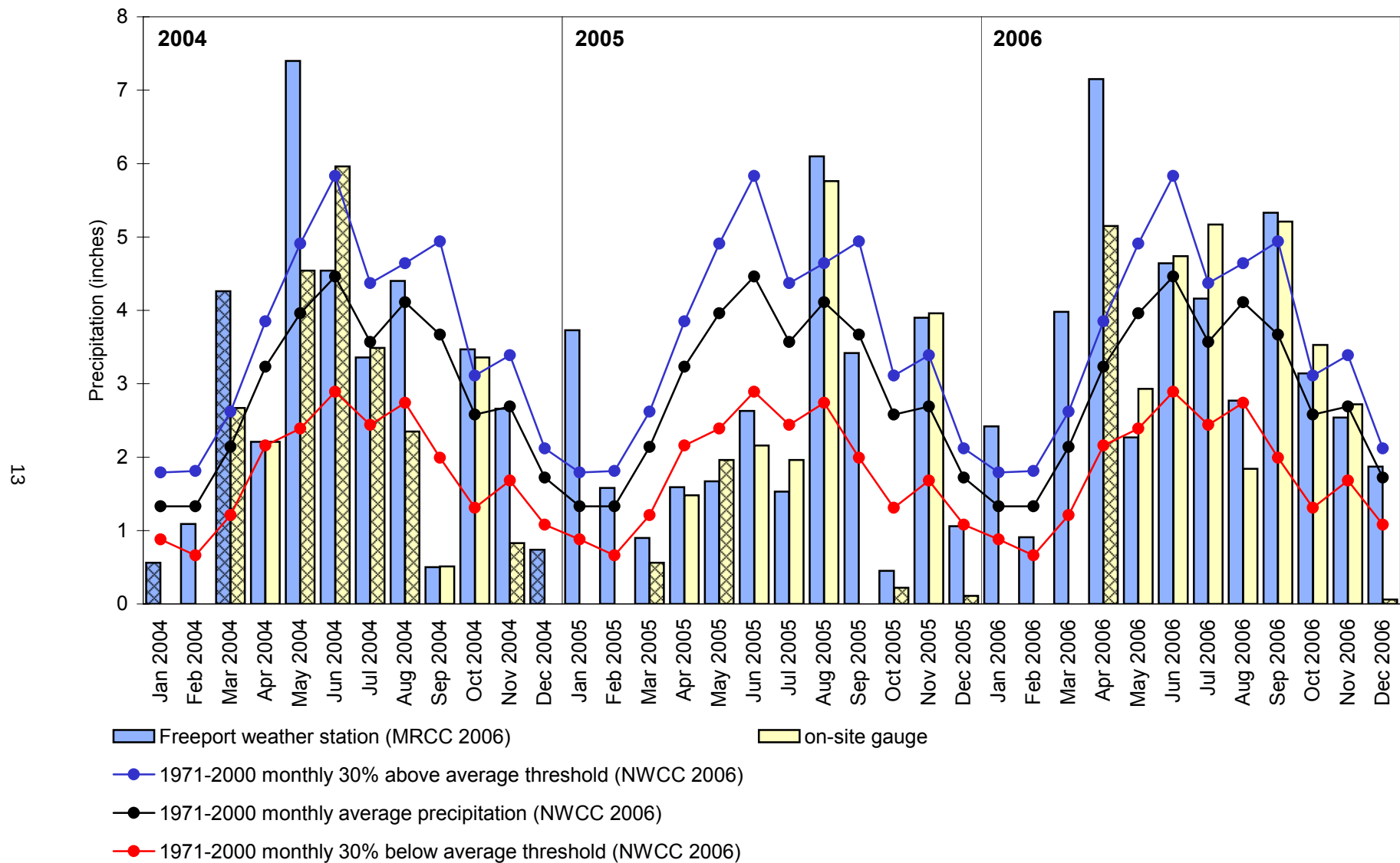
Figure 8 Total monthly precipitation recorded at the Freeport Wastewater Treatment Plant weather station and on site. Incomplete data are indicated with cross-hatching.
