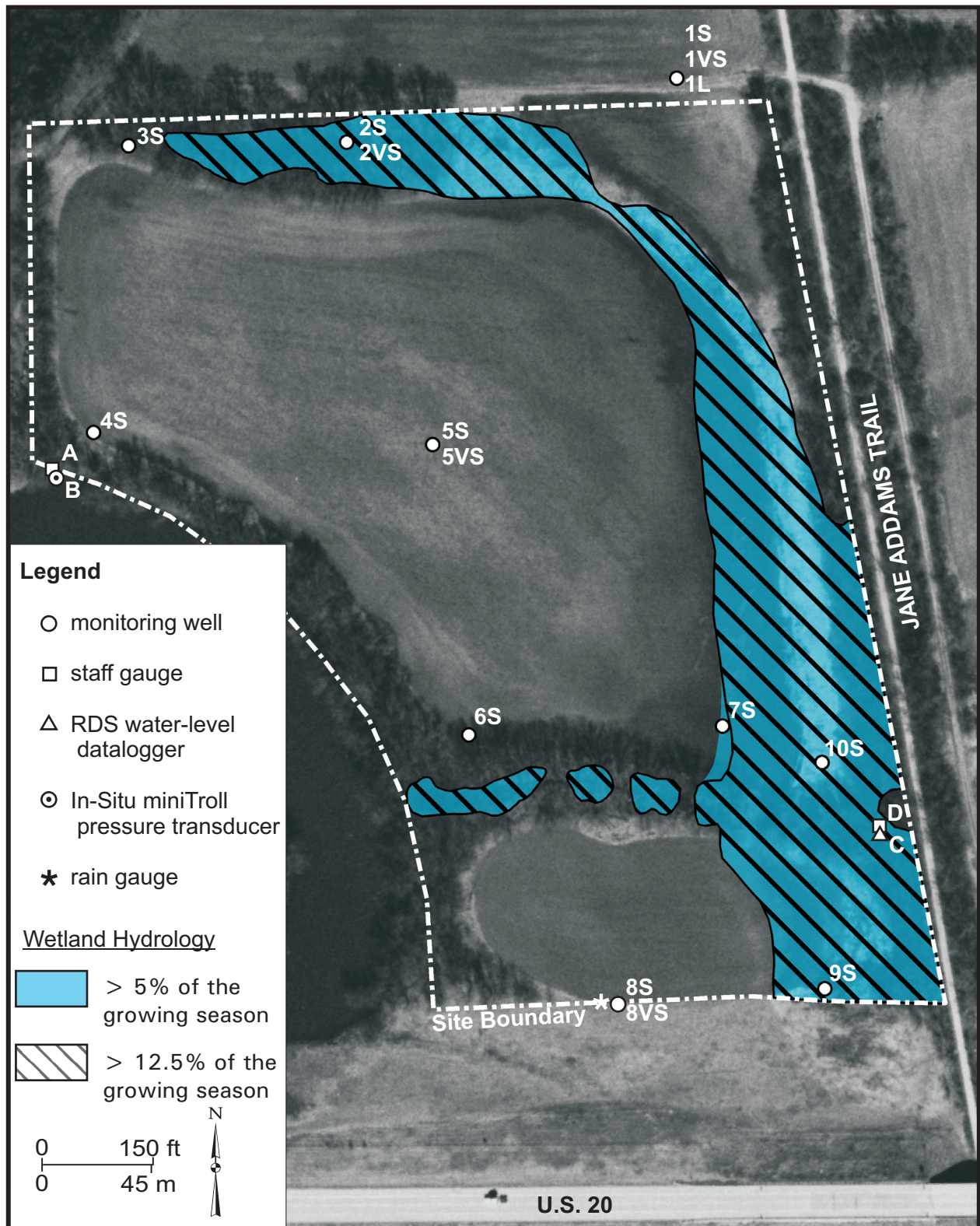
Figure 2 Summary of areas at Site 6W that exhibited wetland hydrology in two out of three growing seasons between 2004 and 2006 (figure based on ISGS 2004, 2005b, and 2006).
