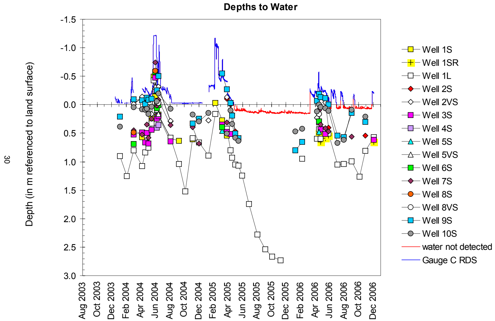
Figure C2 Depths to water in monitoring instruments at the West Freeport Bypass Site 6W.
