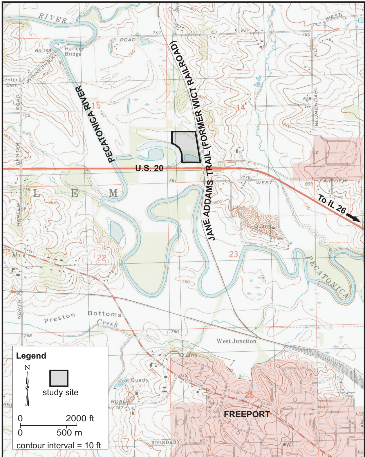
Figure 1 Location of Site 6W, a potential wetland compensation site for the West Freeport Bypass (FAP 301) near the city of Freeport, Stephenson County, Illinois. Figure modified from the Freeport West, IL 7.5-minute U.S. Geological Survey (USGS) Quadrangle (USGS 1998).
