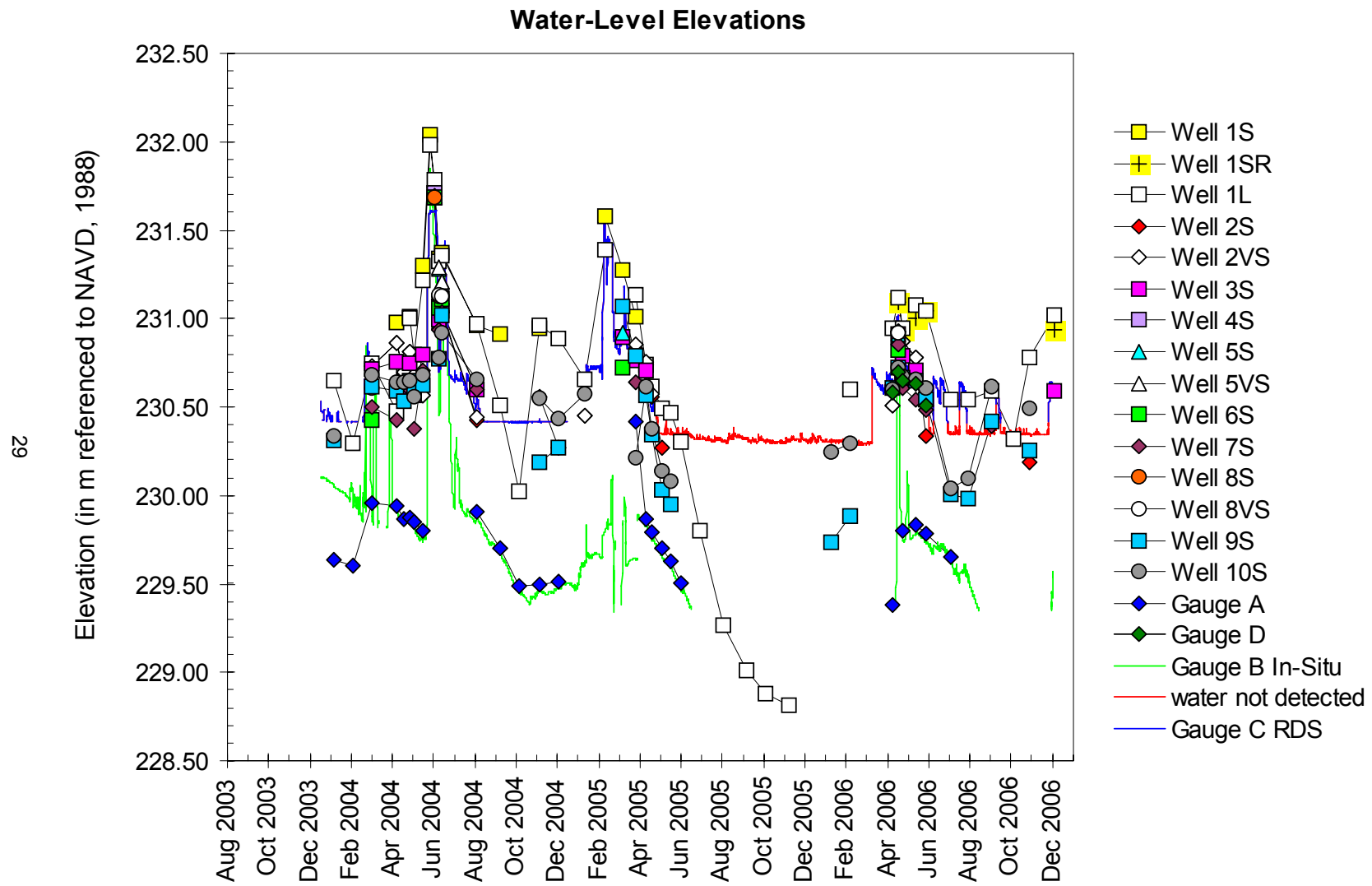
Figure C1 Water-level elevations at monitoring instruments at the West Freeport Bypass Site 6W.
