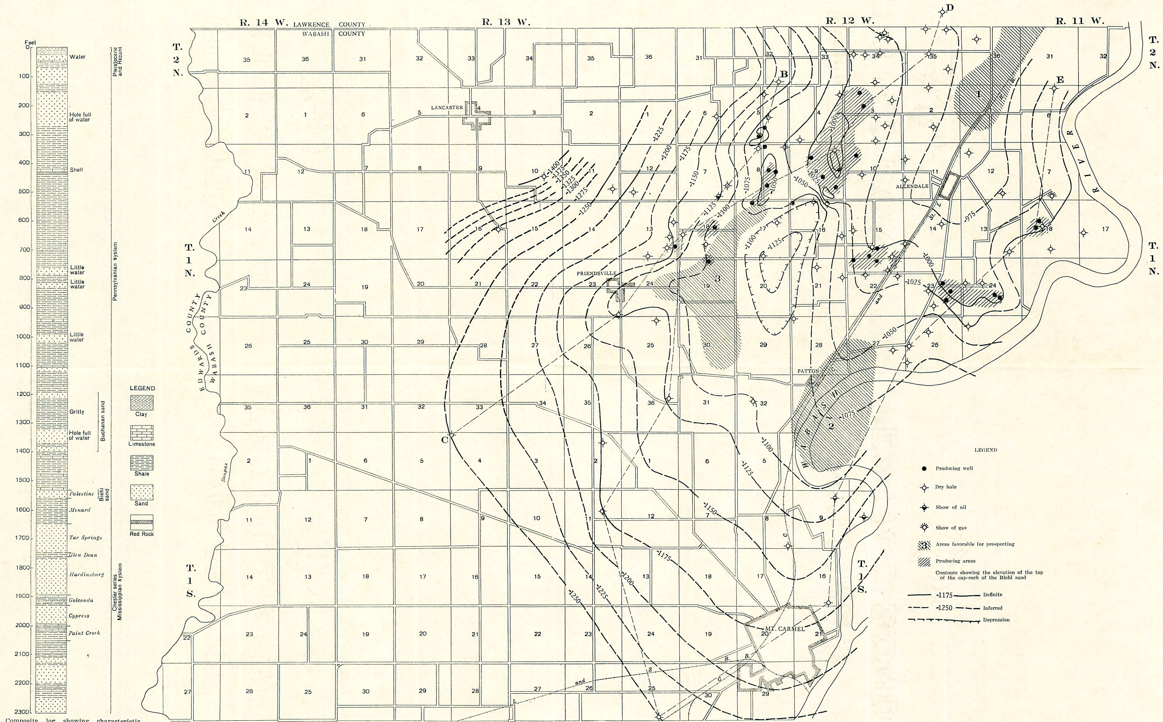
Map of the Allendale area showing structure of the top of the cap-rock of the Bieh1 sand, locations of some of the holes drilled, producing areas, and areas considered favorable for prospecting.
