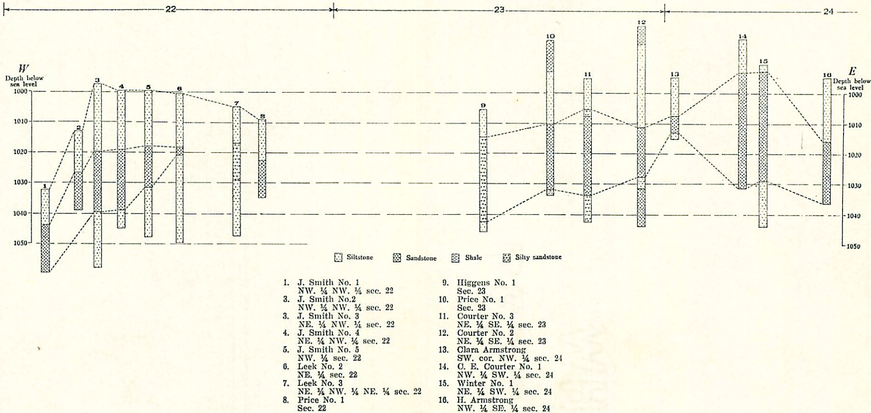
Cross section of the producing zone across secs. 22, 23, and 24, T. 1 N., R. 12 W. (Wabash Twp.) showing the variations in sand conditions and structure.
