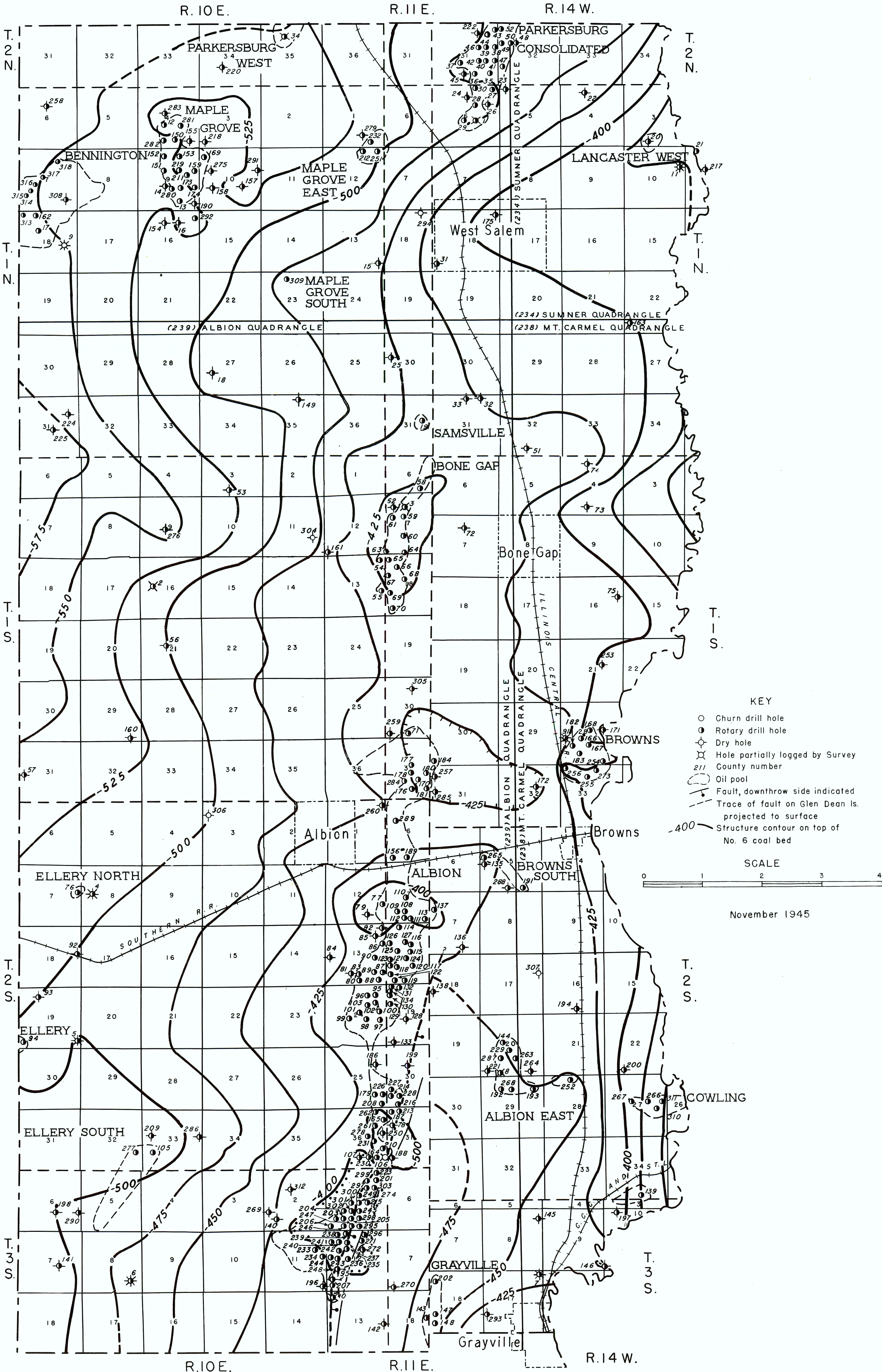
STRUCTURE MAP OF THE TOP OF HERRIN (NO. 6) COAL BED EDWARDS COUNTY
