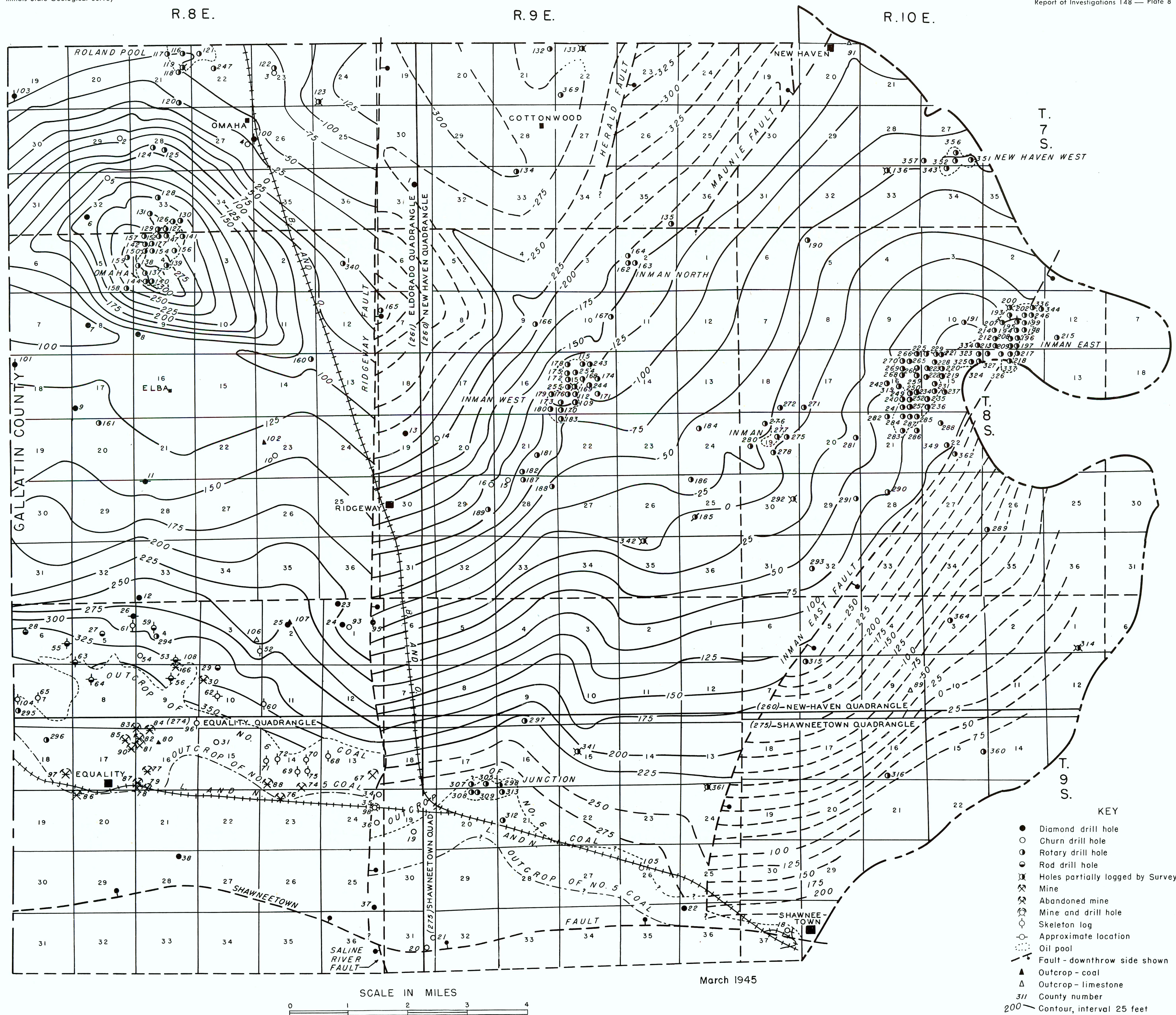
STRUCTURE MAP OF THE TOP OF HERRIN (NO. 6) COAL BED GALLATIN COUNTY
