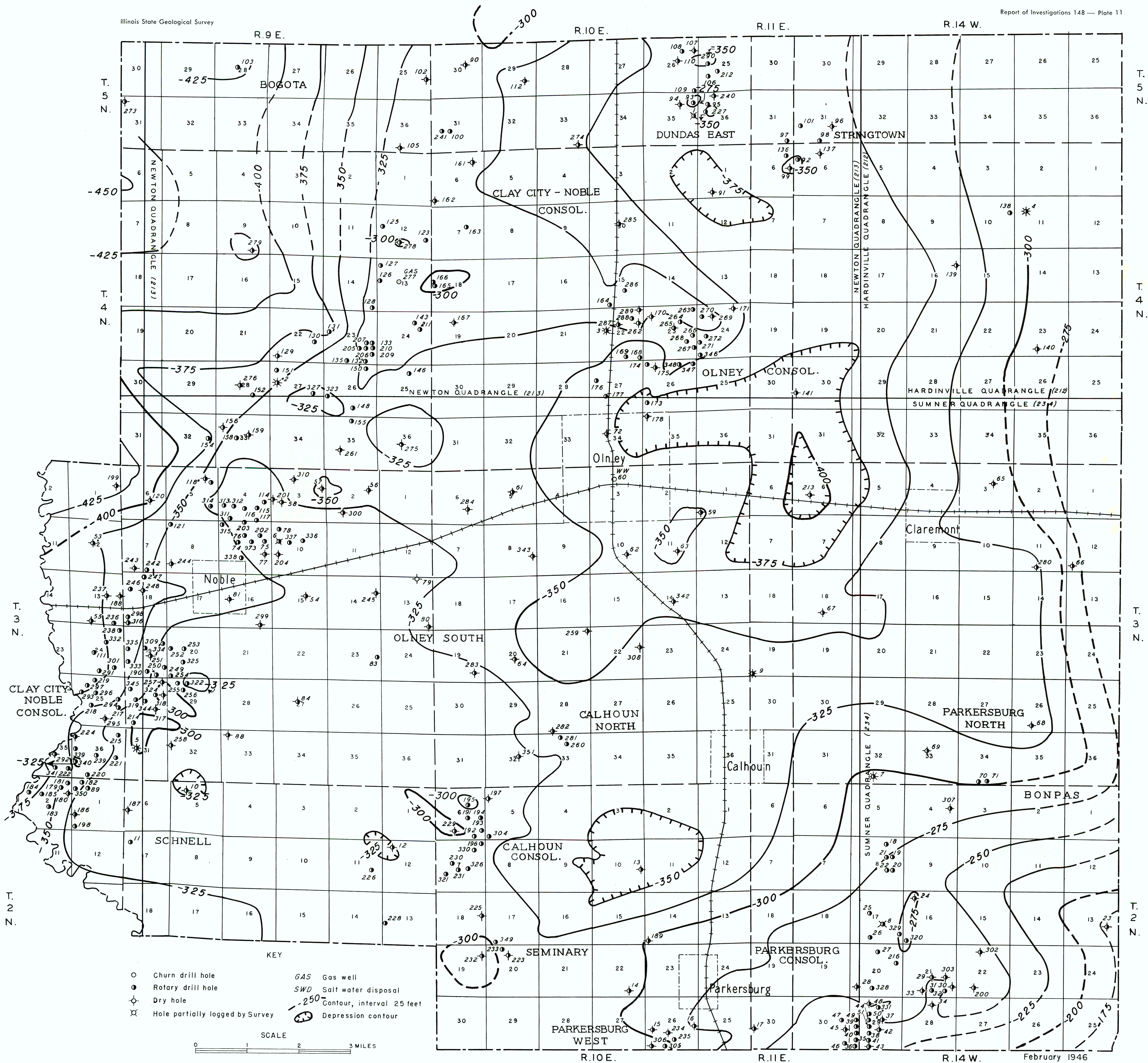
STRUCTURE MAP OF THE WEST FRANKLIN LIMESTONE IN RICHLAND COUNTY
