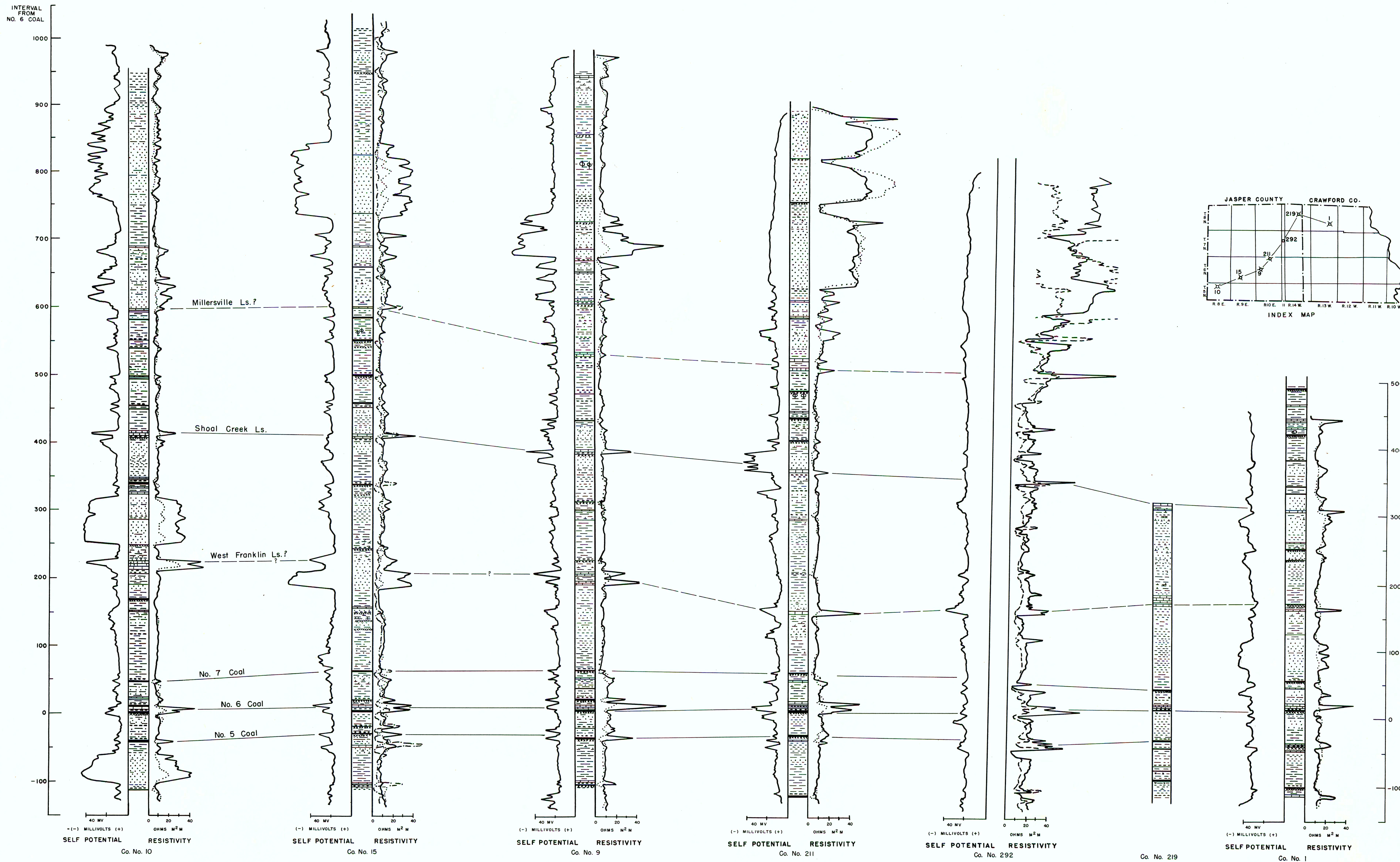
CORRELATION OF PENNSYLVANIAN KEY BEDS IN CERTAIN DRILL HOLES IN JASPER AND NORTHWESTERN CRAWFORD COUNTIES
