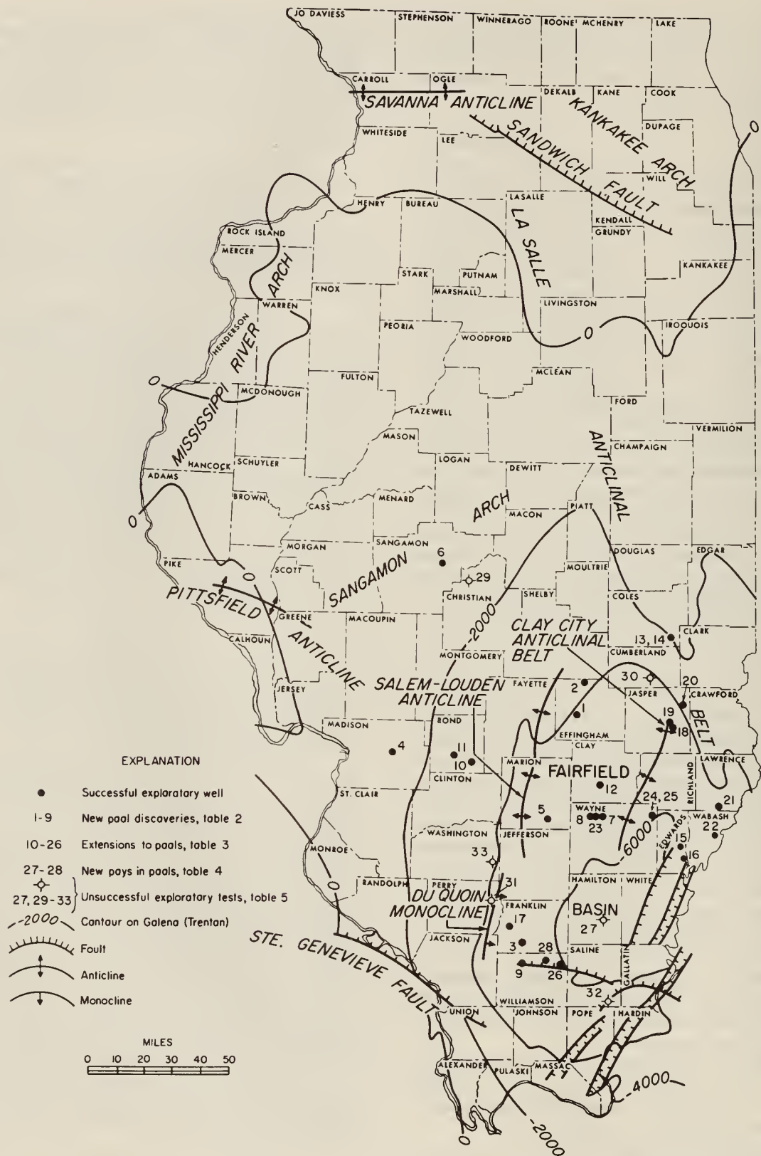
Figure 1 - Major tectonic features of Illinois and their relations to significant holes drilled during 1965. Numbered holes shown are listed in tables 2, 3, 4, and 5.
